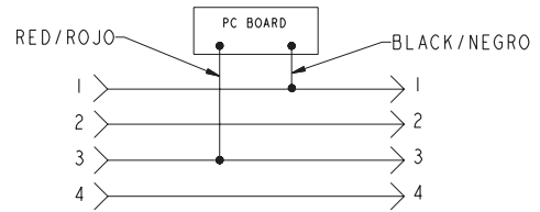
FIG 4 Inline Adapter with Power Diagnostics (114011A-PM-3)
