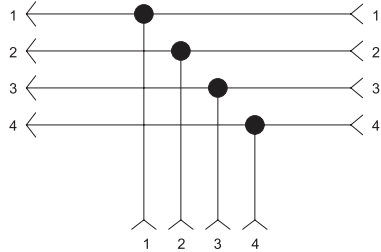
FIG 3 Auxiliary Power Tee (DNAPT)
