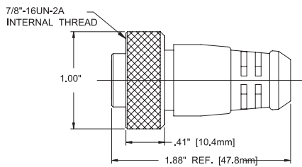
FIG 1 孔座Mini-Change
